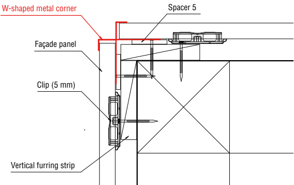
Detail (Clip for horizontal application (5mm))
